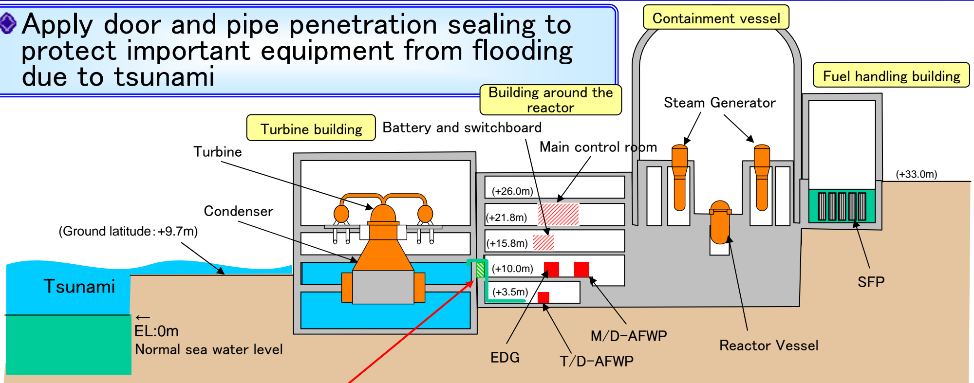
Measures to protect facilities from tsunami
