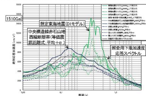
照査用下限加速度応答スペクトル図 © 2014 Chubu Electric Power Co., Inc. All rights reserved. 5
